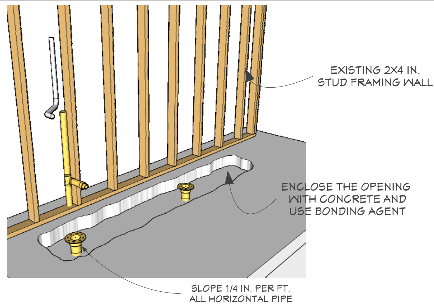
PLUMBING UNDERGROUND PIPE DETAIL (TYP.)
